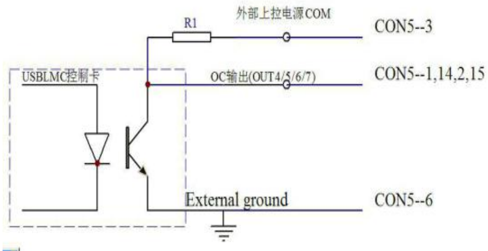
Fig 2-18 normal OC output (OUT4/5/6/7) , R1 is inductive load.
