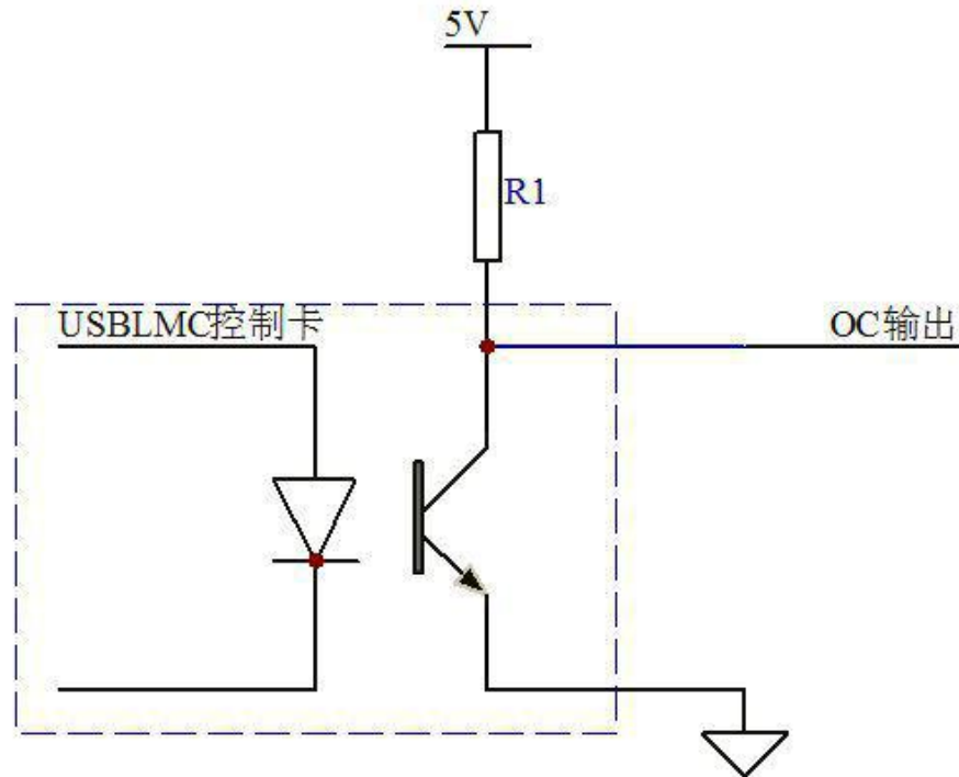
Fig 2-17 Normal OC output (OUT10/OUT11/OUT12)
