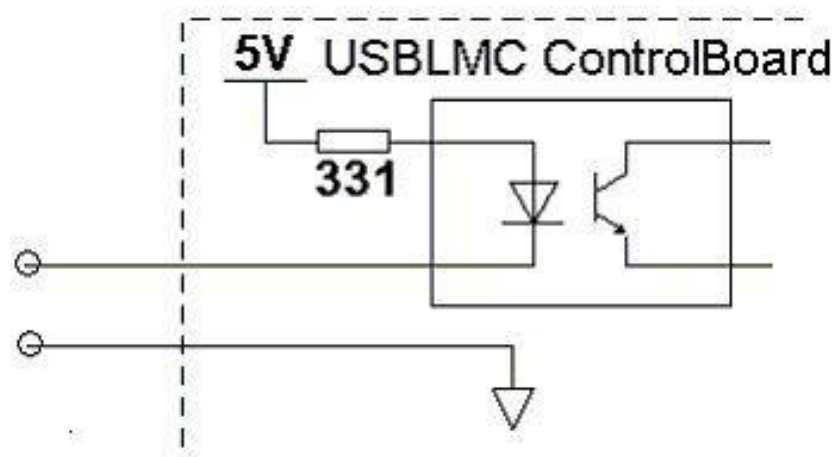
Pic 2-7 wiring for general input pins
