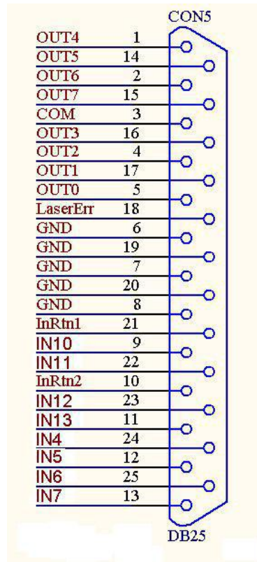
Pic 2-5 CON5 pin definition
