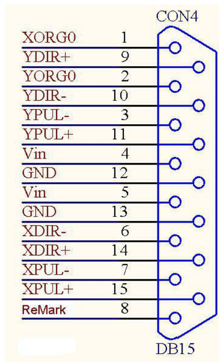
Pic 2-4 CON4 pin definition
