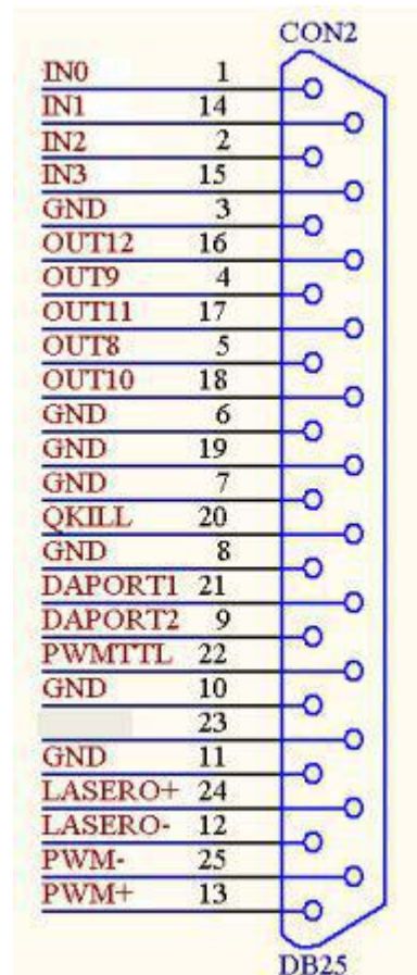
Pic 2-2 CON2 pin definition
