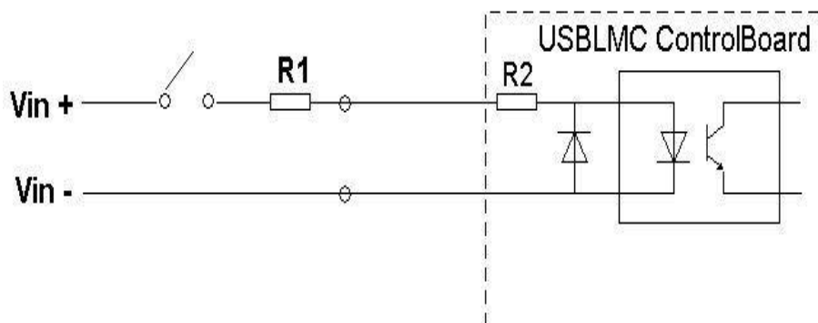
Pic 2-10 recommended wiring for general input pin in9
