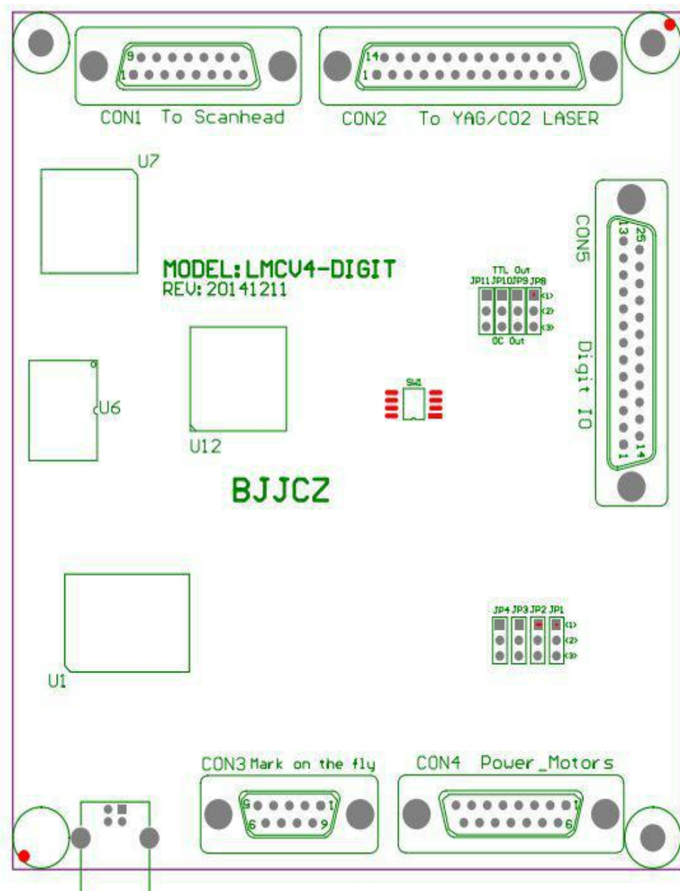
Fig1- 1 LMCV4-DIGIT digital card illustration
