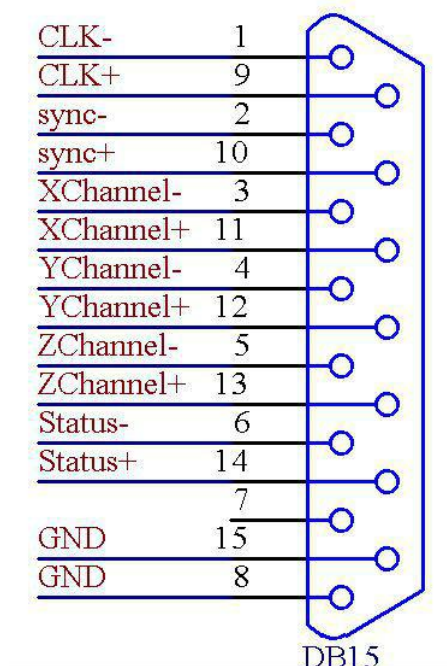
Pic 2- 1 CON1 pin definition
