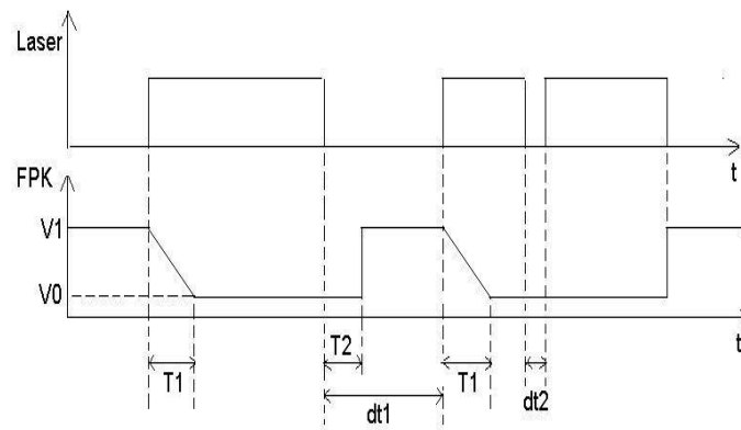
Fig.1-13-3 Analog FPK
